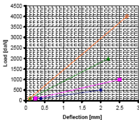
Load/Deflection Chart for ZAL MOUNTS
